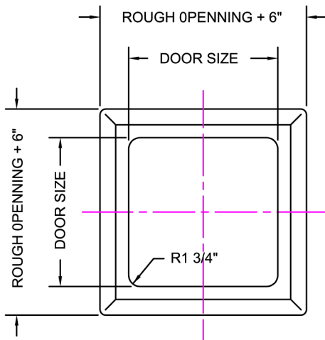
Drop-in Access Panel -Type Panel Elevations
